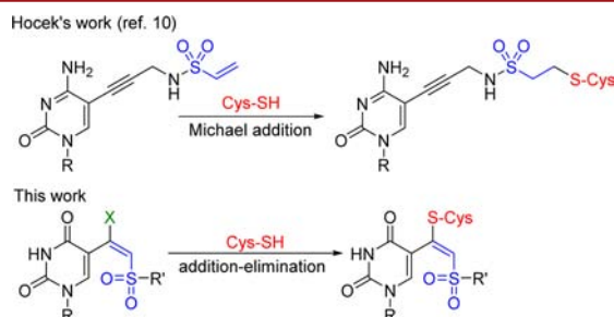
Figure 1. Bioconjugation of uracil-based vinyl sulfones with thiolates via the Michael addition 10 or conjugated addition–elimination.
