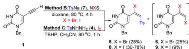
Scheme 3. Synthesis of 5-( \beta -Halo)vinyl Sulfones via NXS-Catalyzed Halosulfonylation of 1 with 7 or TBHP-Promoted Halosulfonylation of 1 with 4
