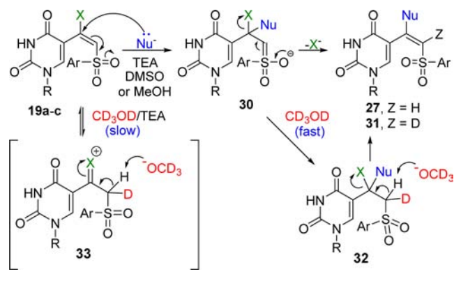
Scheme 4. Plausible Mechanism for the Nucleophilic Substitution of Halides from Uracil 5-( \beta -Halo)vinylsulfones
