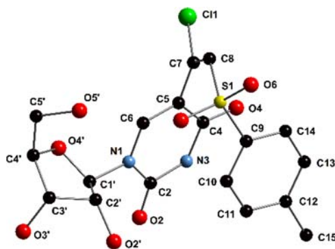
Figure 2. X-ray crystal structure of E - 19a . H atoms and interstitial H 2 O molecules are omitted for clarity.
